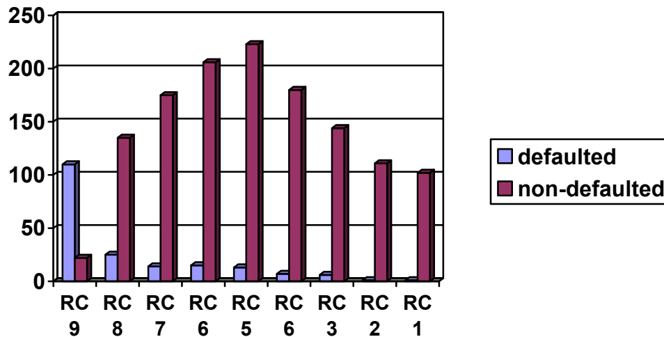
Fig. 1: Histogram of defaulted and non-defaulted exposures in 9 rating classes
