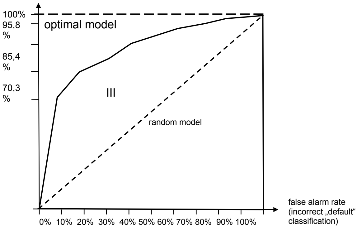
Fig. 3: ROC Curve
