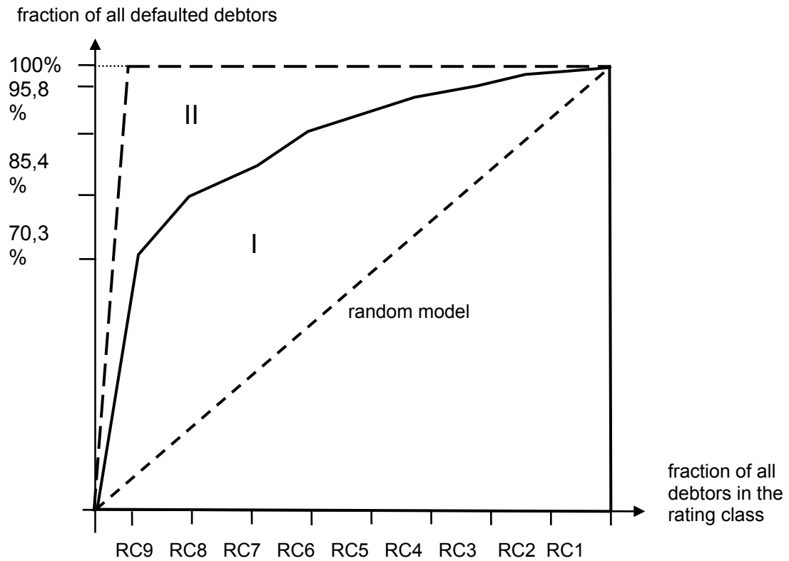
Fig. 2: Lorenz Curve
